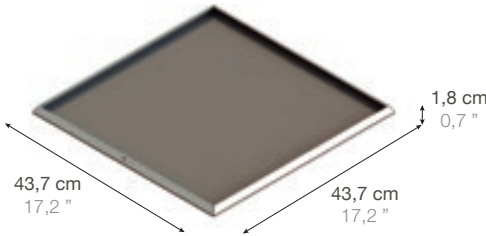
GRIDDLE / PLANCHA
